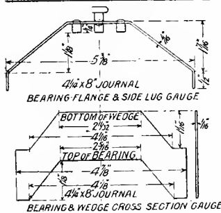
BEARING & WEDGE CROSS SECTION GAUGE
